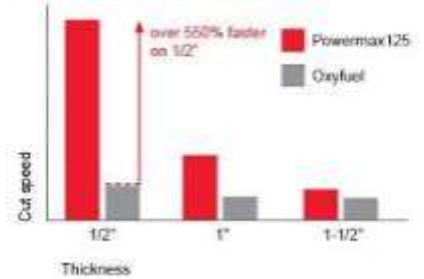
Relative cut performance on mild steel
