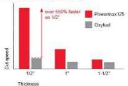
Relative cut performance on mild steel
